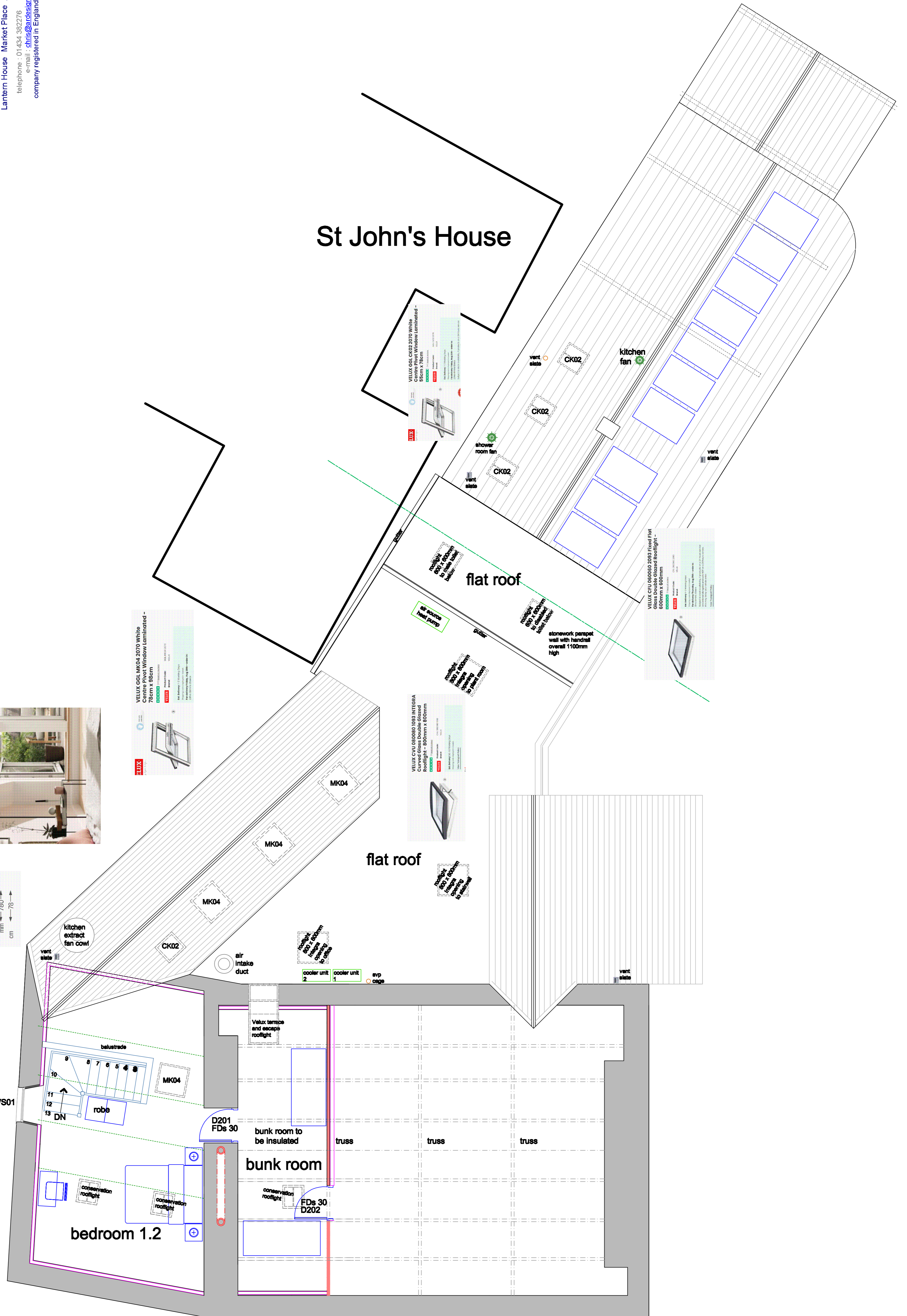
SECOND FLOOR PLAN AS PROPOSED
